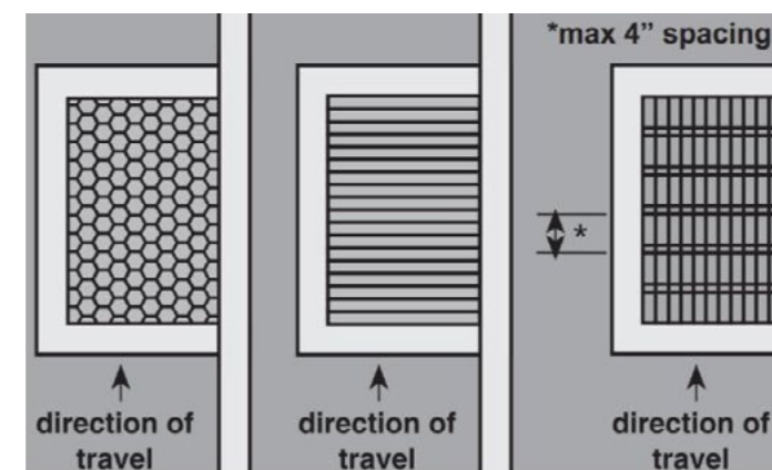
Bicycle Safer Grates - Oregon Bicycle & Pedestrian Guide
