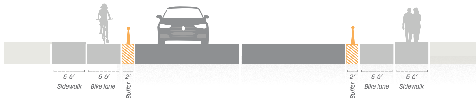
FIGURE 9. FLEXIBLE DELINEATES OR BOLLARDS
