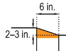
Mountable curb, AASHTO Bicycle Facilities, 5th Edition
