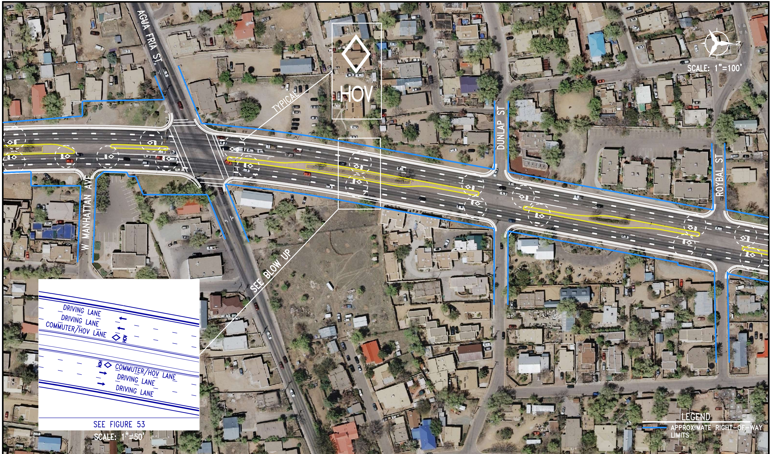
FIGURE 39 LANE CONVERSION TO DEDICATED COMMUTER/HOV LANE
