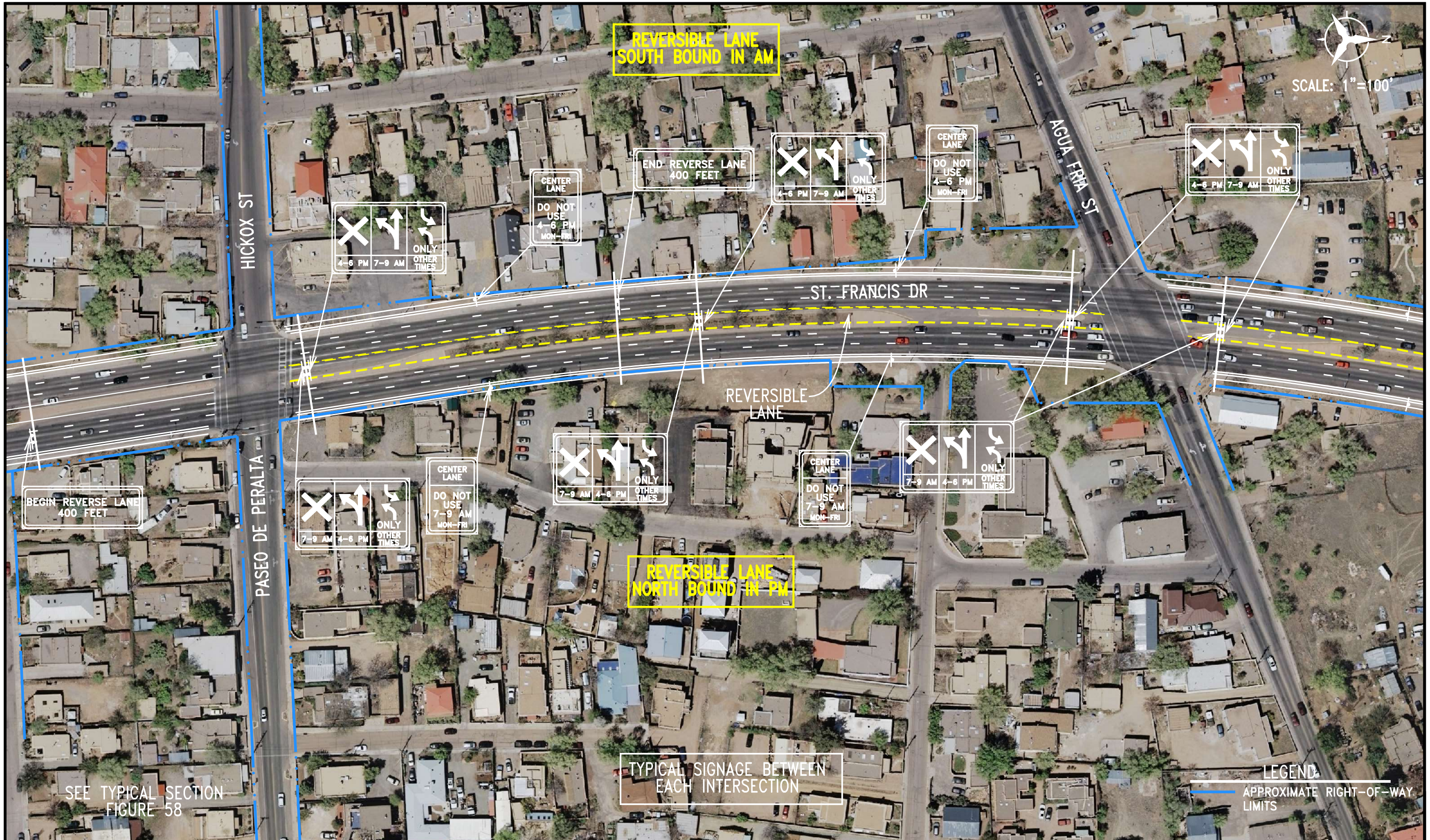
FIGURE 42 LANE CONVERSION TO REVERSIBLE LANE (CITY TRAFFIC COMMUTER)
