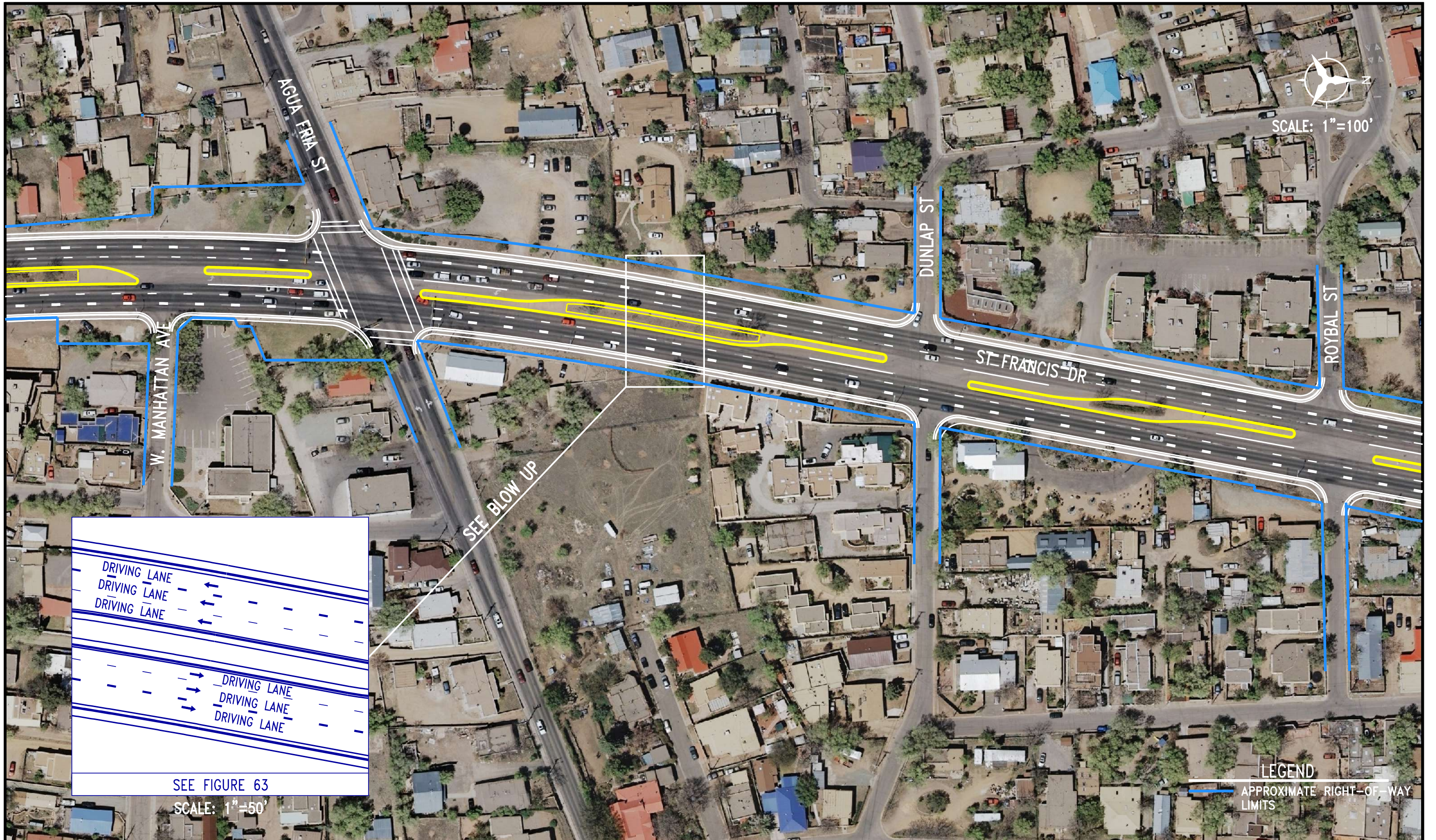
FIGURE 44 REDUCED LANE WIDTH
