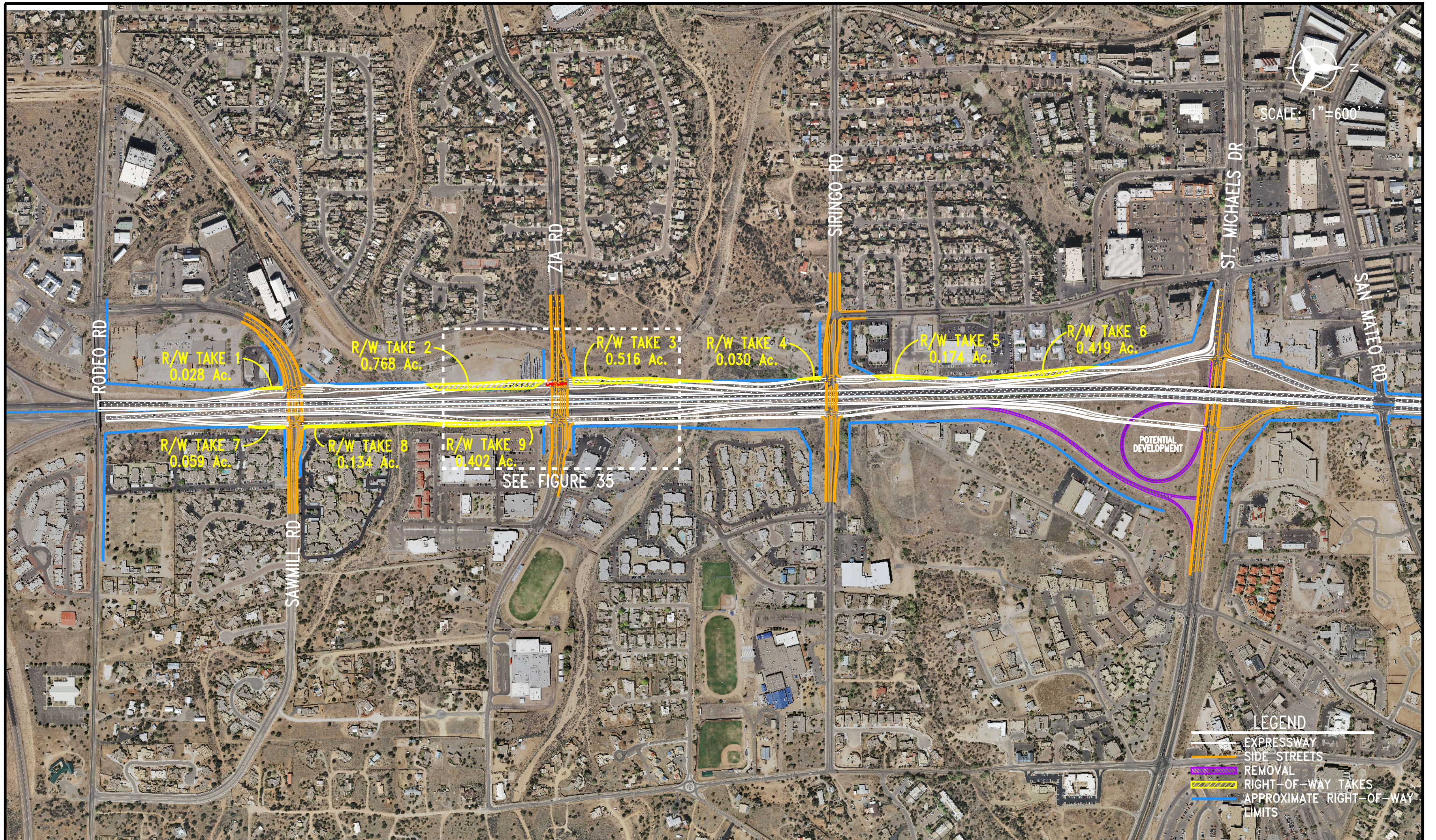
FIGURE 54 EXPRESSWAY WITH FRONTAGE ROAD THROUGHOUT SOUTH END OF CORRIDOR
