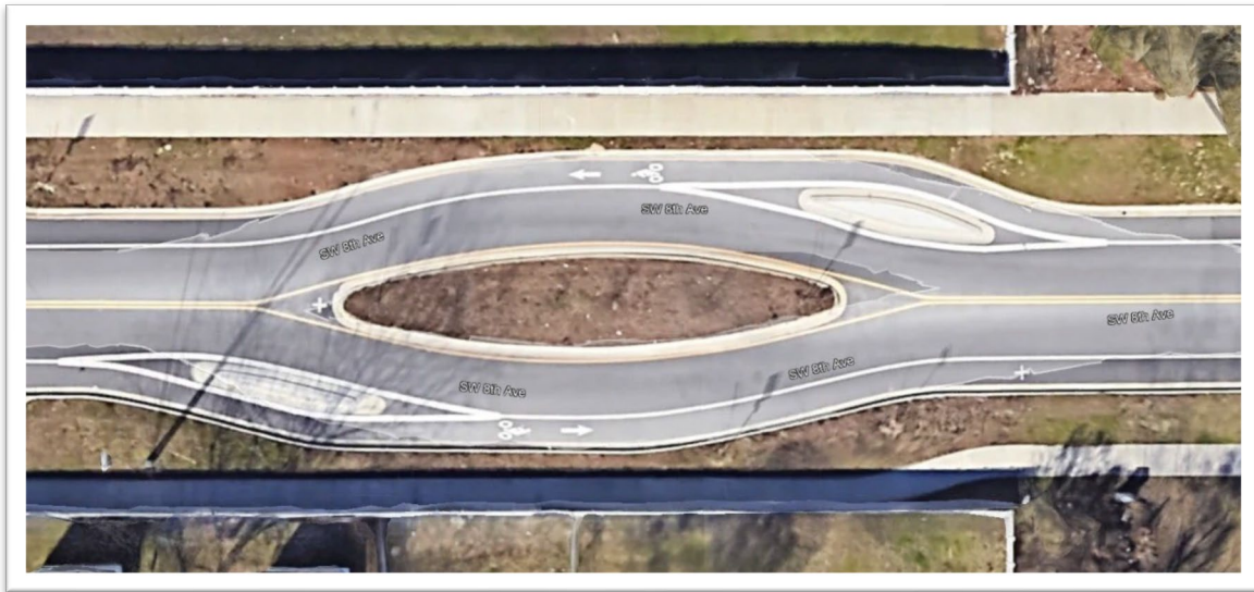
Figure 35: Median Island on a Two-Lane Road with Bicycle Lanes
