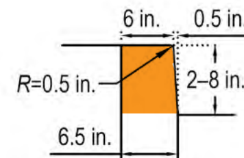
Vertical curb, AASHTO Bicycle Facilities, 5th Edition
