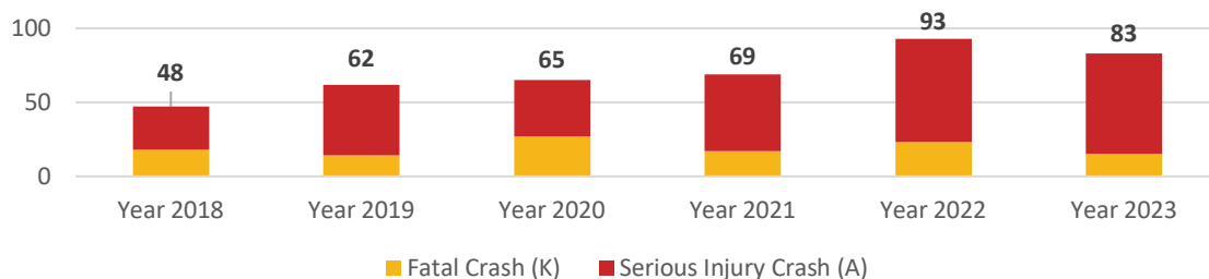
FIGURE 4-17. SEVERE CRASHES PER YEAR, 2018-2023
