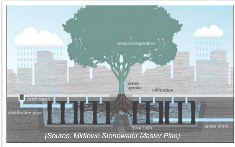
Figure 11: Suspended Pavement Cell System Overview, Deeproot
